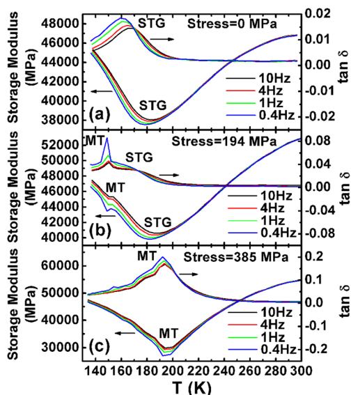
FIG. 2. (Color online) The dependence of internal friction and associated storage modulus of \text{Ti}_{48.8}\text{Ni}_{51.5} strain glass on bias stress of (a) 0 MPa, (b) 194 MPa, and (c) 385 MPa. The results are measured with multi-frequency from 0.4 Hz to 10 Hz. They show that the change of the transforming route of strain glass upon stress leads to the stress changed damping behavior. The STG and MT in the figure represent the strain glass transition and the martensitic transition, respectively.
