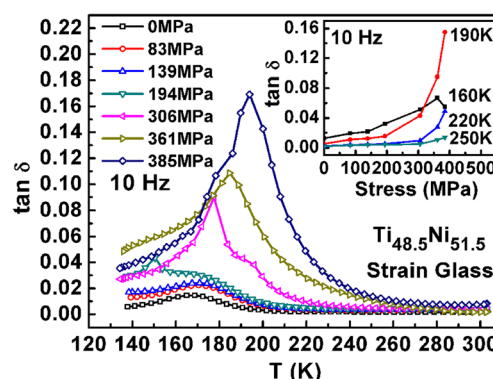
FIG. 1. (Color online) Stress changed damping behavior for \text{Ti}_{48.5}\text{Ni}_{51.5} strain glass. The inset shows that the internal friction value of this sample can be changed greatly by bias stress in the temperature range from 160 K to 250 K. The testing frequency is 10 Hz.
